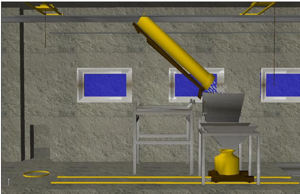
WITNESS VR - 3D Model of the Basket Handling Cave showing a basket of hulls being tipped into a hulls container
