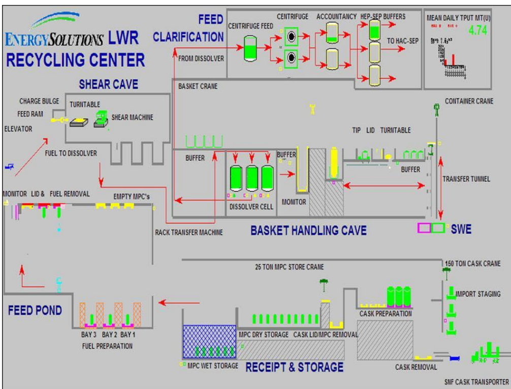
The WITNESS 2D Model display of the Head End Plant which including Fuel Receipt and Storage, Feed Pond, Shear Cave, Basket Handling Cave and Feed Clarification
