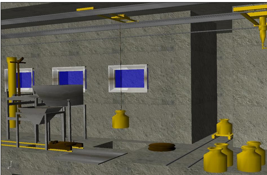
WITNESS VR - 3D Model of the Basket Handling Cave showing a hulls container being exported using a crane.
