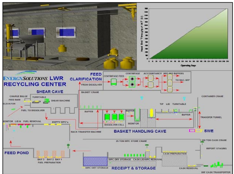
Picture of WITNESS 2D and 3D displays and an output graph from the model.
